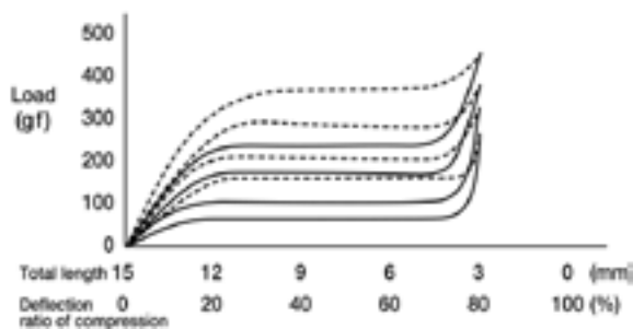
Stress Strain curves opened spring
